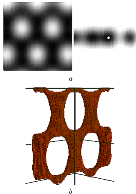
Fig. 6. Distributions of valence electron density for the 5-zGNR: longitudinal cross-section through the centers of atoms (left panel) and transverse cross-section in a vicinity of the C atom the most distant from the edges (right panel) (a); spatial distribution of valence electron density within the interval of 0.8–0.9 of the maximum value for the C atom the most distant from the edges (b)
