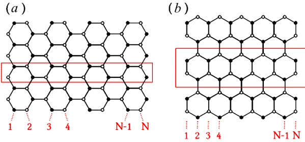
Fig. 2. Carbon N -aGNRs (a) and N -zGNRs (b) composed of N armchair or zigzag lines, respectively. White and black circles identify carbon atoms related to two different sublattices, A and B. Rectangles confine unit cells in corresponding GNRs. The enumerated atoms correspond to the number of zigzag chains or dimer lines across the nanoribbon width
