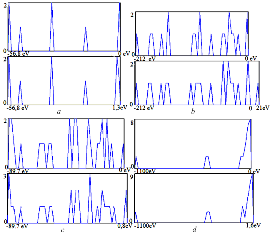
Fig. 3. Distributions of states at the \Gamma -point of the Brillouin zone in a superlattice that simulates the graphene plane (a), the 5-zGNR (b), the 7-zGNR (c), and the 7-zGNR with hydrogen-decorated edges (d). The upper distribution in the group corresponds to the valence band states and the lower one to the valence band states and the next allowed state. The energy in electron volts is reckoned along the abscissa axis, and the number of states is shown on the ordinate axis
