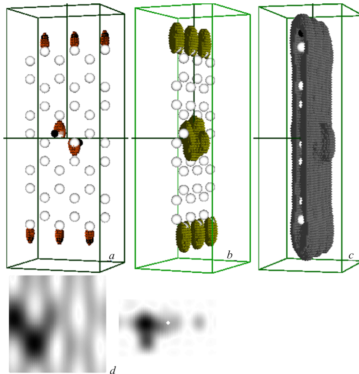
Fig. 9. Distribution of valence electron density within the interval of 0.8–0.9 of the maximum value in a unit cell of the 7-zGNR with H-decorated edges and adsorbed H atoms (to a concentration of 4.8%) at positions located on the different sides from the graphene plane over the neighbor C atoms that are the most distant from the edges ( a ). The same as in panel a , but for the concentration intervals of 0.5–0.6 and 0.1–0.2, respectively, of the maximum value ( b ) and ( c ). Longitudinal and transverse cross-sections of the spatial distribution in a vicinity of the C atom with a hydrogen atom being adsorbed above ( d )
