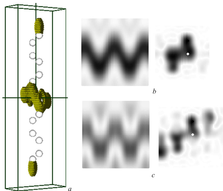
Fig. 8. Distribution of valence electron density within the interval of 0.5–0.6 of the maximum value in a unit cell of the 7-zGNR with H-decorated edges and adsorbed H atoms (to a concentration of 14.3%) at positions located on the different sides from the graphene plane over the neighbor C atoms that are the most distant from the edges ( a ). Longitudinal and transverse cross-sections of the spatial distribution in a vicinity of the C atom with a hydrogen atom being adsorbed above ( b ) and in a vicinity of the same C atom, but in the GNR with an additionally adsorbed O atom at the position that is nearest to this C atom (above the neighbor carbon atom) ( c )
