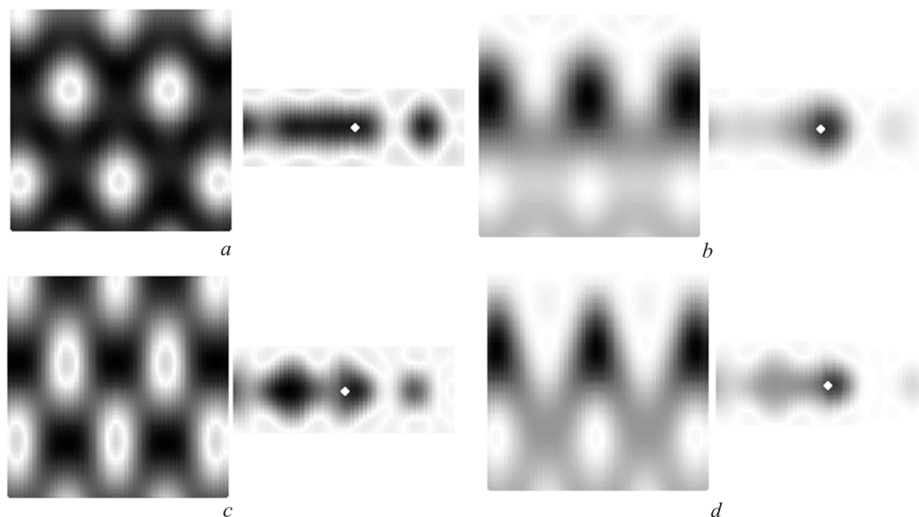
Fig. 7. Longitudinal and transverse cross-sections of the spatial distributions of valence electron density for the 5-zGNR with hydrogen-decorated edges ( a ) in a vicinity of the C atoms the most distant from the edges and ( b ) in a vicinity of the C atoms that confine the ribbon and interact with hydrogen atoms. Panels ( c ) and ( d ) illustrate the same distributions for the same positions of atoms described above, but for the 7-zGNR
