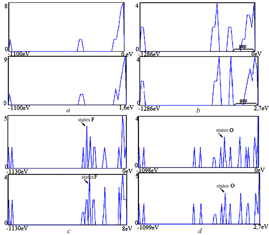
Fig. 4. Distributions of states at the \Gamma -point for the 7-zGNR with H-decorated edges (a); the same GNR as in panel (a), but with two additional H atoms located above the neighbor C atoms on the different sides from the GNR plane (b); for the same GNR as in panel (b), but with two additional F atoms located over C atoms on the different sides from the GNR plane at positions that are the nearest to H atoms (c); for the same GNR as in panel (c), but with two additional O atoms instead of F ones (d). In each group of distributions, the upper distribution corresponds to valence band states, and the lower one to valence band states and the next allowed state. The energy in electron volts is reckoned along the abscissa axis, and the number of states is shown on the ordinate axis
