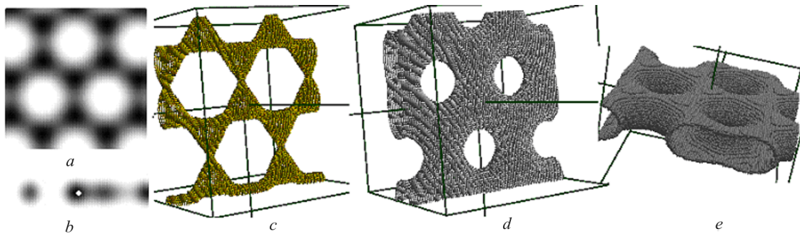
Fig. 5. Longitudinal (a) and transverse (b) cross-sections of the spatial distribution of valence electron density over an unconfined graphene plane drawn through the centers of atoms, spatial distribution of valence electron density within the interval of 0.6–0.7 of the maximum value (c); the same as in panel (c), but for the interval of 0.1–0.2 of the maximum value exposed in different perspectives (d) and (e)
