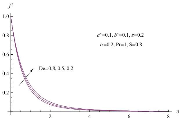
Fig. 5. Behavior of the velocity distribution for various values of De
