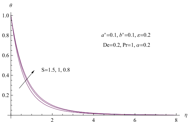
Fig. 4. Behavior of the temperature distribution for various values of S
