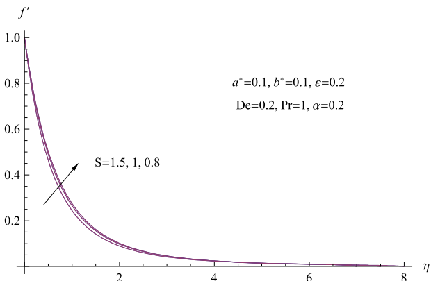
Fig. 3. Behavior of the velocity distribution for various values of S
