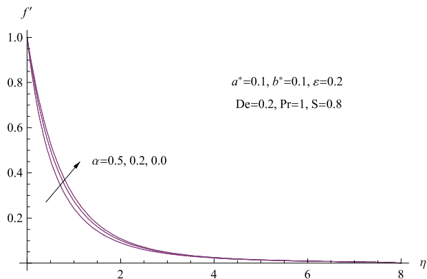
Fig. 8. Behavior of the velocity distribution for various values of \alpha
