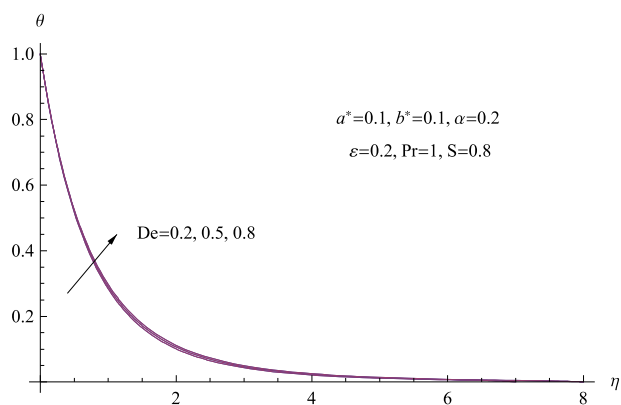
Fig. 6. Behavior of the temperature distribution for various values of De
