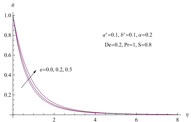
Fig. 10. Behavior of the temperature distribution for various values of \varepsilon
