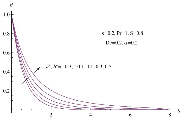
Fig. 11. Behavior of the temperature distribution for various values of a^* , b^*
