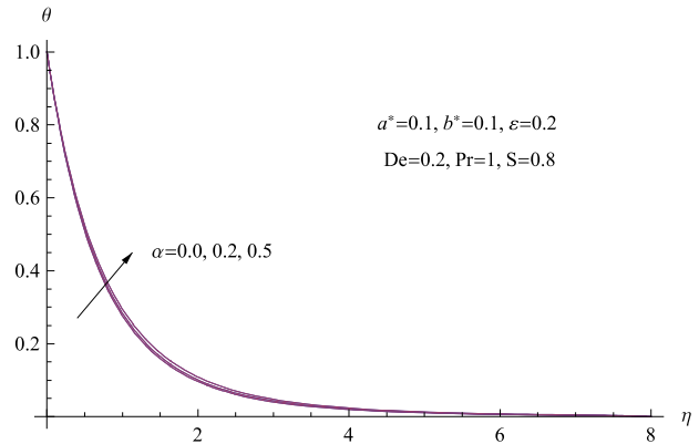
Fig. 9. Behavior of the temperature distribution for various values of \alpha
