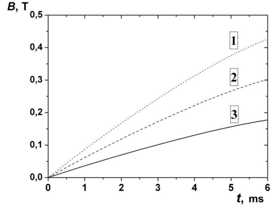
Fig. 3. Time dependence of the magnetic field induction. U_B = 2 (1), 1.4 (2), and 0.84 kV (3)
