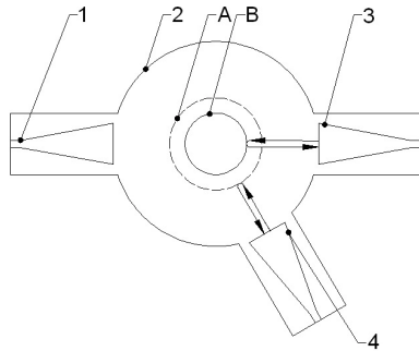
Fig. 4. Diagram of the arrangement of antennas for correlation and interferometric measurements: (1) receiving antenna of interferometer, (2) vacuum chamber, (3 and 4) transmit-receive antennas of a reflectometer. A and B are plasma layers with N_p = N_{cr}^{1,2} .
