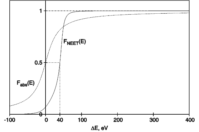
NEET edge function F_{\text{NEET}}(E) (solid) and K-absorption factor F_{\text{abs}}(E) (dashed), calculated for nucleus ^{197}\text{Au} , versus the energy E of x-ray photons, where \Delta E = E - B_K , and B_K denotes the binding energy of the K-electron
