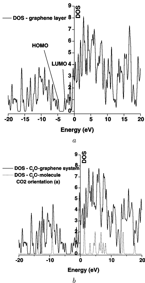
Fig. 4. DOS for a pristine graphene sheet and a graphene sheet adsorbed with a CO 2 molecule on the adsorption site (a)
