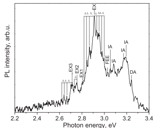
Fig. 3. PL spectrum of rutile sample
