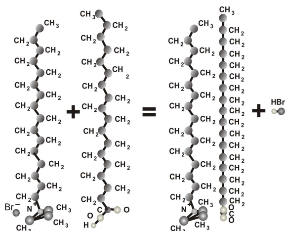
Fig. 1. Schematic representation of the formation of possible bitail CA supramolecular structure in a reaction between a cationic (CTAB) and anionic (SA) compounds
