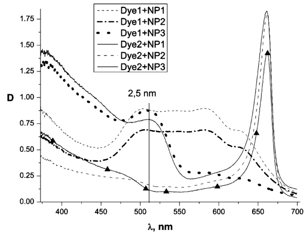
Fig. 5. Absorption spectra of dyes 1 and 2 conjugated with nanoparticles with diameters of 1.2, 1.1, and 2.3 nm; 4 months after the preparation
