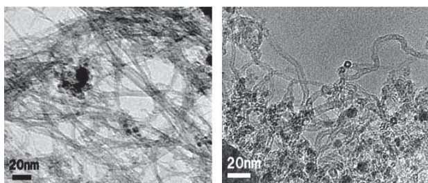
Fig. 2. Transmission electron micrographs of synthesized carbon fine particles
