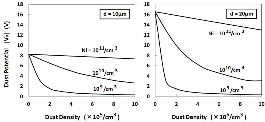
Fig. 5. Dust density dependence of the dust floating potential in plasma with ion densities of 10^{11}/\text{cm}^3 , 10^{10}/\text{cm}^3 , and 10^9/\text{cm}^3 for spherical dusts of 10 and 20 microns in diameter. The electron temperature and ion temperatures are assumed 5 eV and 0.1 eV, respectively
