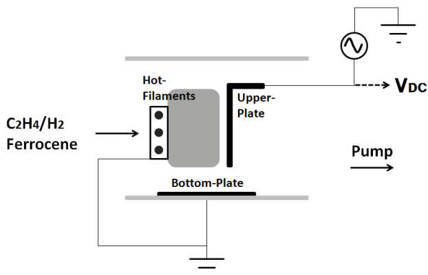
Fig. 1. Schematic diagram of the RF glow discharge plasma system with hot-filaments
