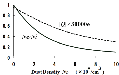
Fig. 4. Dust density dependence of Q and N_e/N_i under the conditions of N_i = 10^{10}/\text{cm}^3 and a spherical dust size of 10 microns. The electron and ion temperatures are assumed 5 eV and 0.1 eV, respectively
