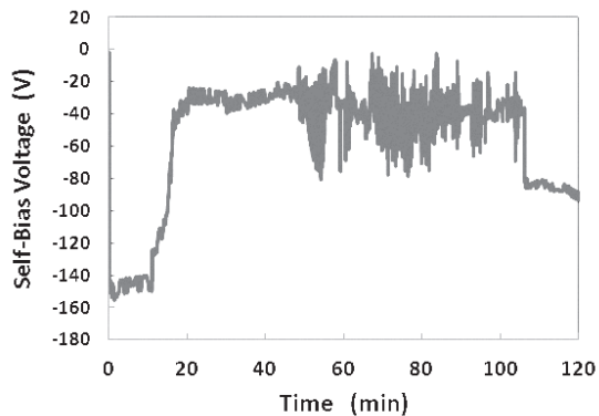
Fig. 3. Variation of the self-bias voltage during the fine-particle growth
