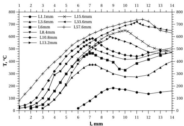
Fig. 6. Temperature distributions in the horizontal cross-sections of the enriched flame at different heights along the flame's axis
