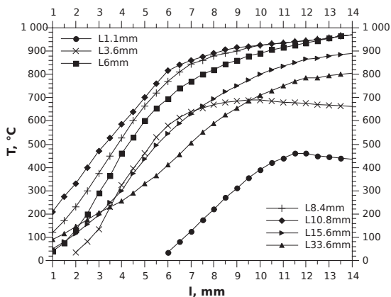
Fig. 7. Temperature distributions in the horizontal cross-sections of the diluted flame at different heights along the flame's axis
