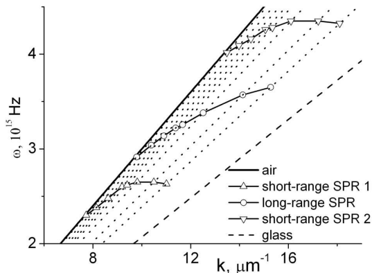
Fig. 5. Dispersion characteristics \omega(k) of the SPR in an Au film with d = 50 nm
