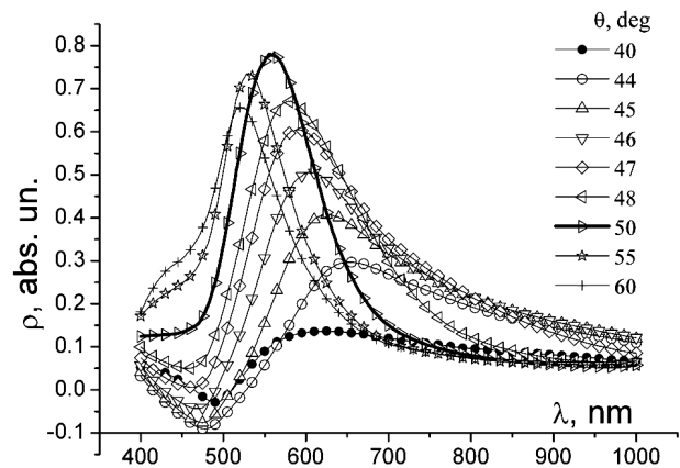
Fig. 1. Evolution of the \rho_{\theta}(\lambda) -spectra for an Au film with d = 50 \text{ nm} associated with the variation of the light incidence angle
