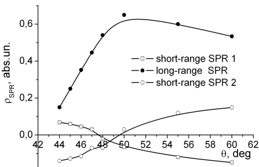
Fig. 6. Dependences of the amplitudes of Gaussian-like components that approximate the normalized \rho_{\text{SPR}} on the light incidence angle
