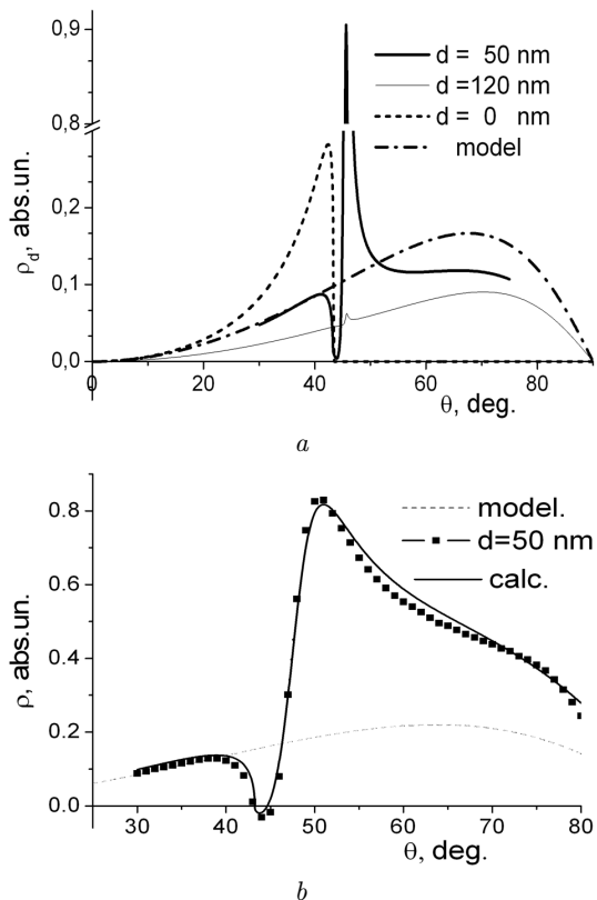
Fig. 2. (a) Dependences \rho(\theta) at \lambda = 632 nm for Au films of various thicknesses and the model non-resonant component for a film with d = 50 nm. (b) The same as in panel (a) but for a film with d = 50 nm at \lambda = 550 nm: experimental and theoretical dependences, and its non-resonant component (dashed curve)
