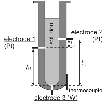
Fig. 1. Scheme of the experimental capillary cell
