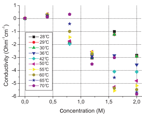
Fig. 4. Concentration dependence of the difference between the conductivities of DNA and electrolyte solutions
