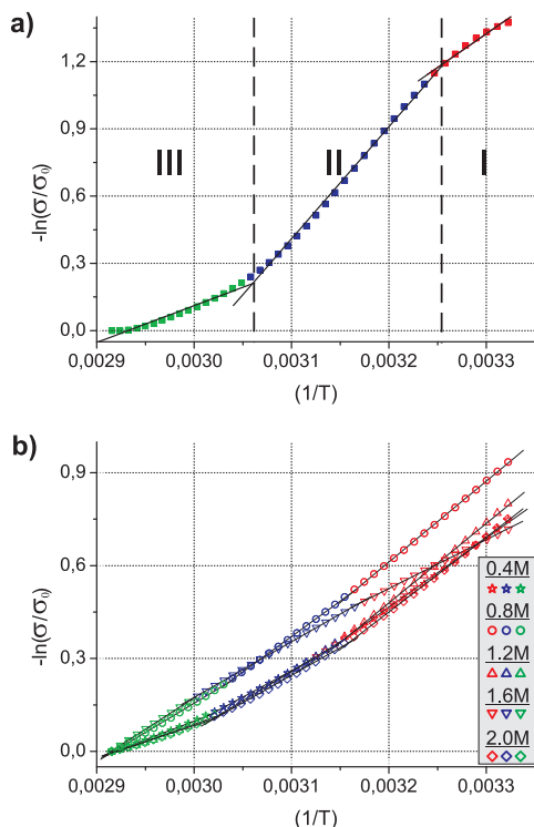
Fig. 3. Arrhenius plot for DNA water solutions. a – salt-free solution. Range I corresponds to a double-stranded DNA (red points); II is the transition range of the double helix melting (blue points); Range III corresponds to a single-stranded DNA (green points). b ) – solution of DNA with added salt. Solid black lines is the linear approximation
