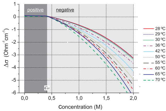
Fig. 5. Dependence of the difference between the conductivity of DNA and that of the electrolyte solution on the salt concentration calculated by formula (12)
