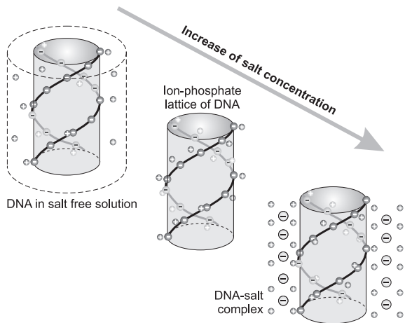
Fig. 6. Scheme of the process of ionic structuring around a DNA double helix at different concentrations of added salt
