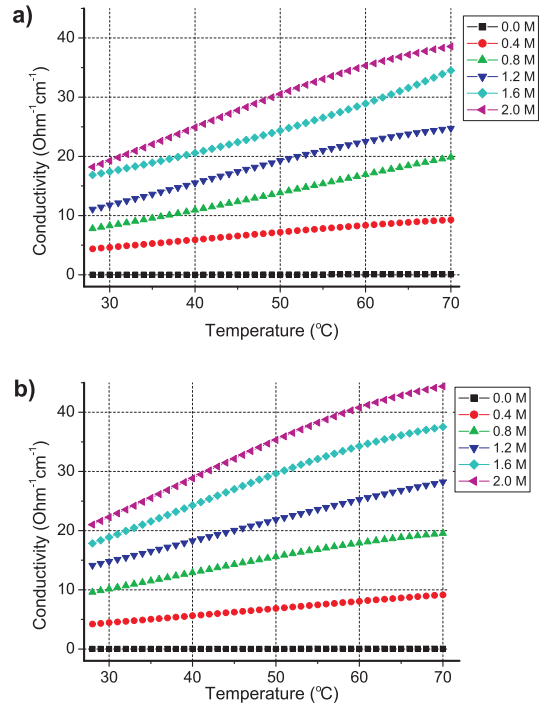
Fig. 2. Temperature dependence of the electrical conductivity of the samples: a) DNA solution with added KCl salt; b) KCl solution
