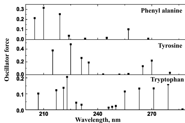
Fig. 4. Electronic absorption spectra of aromatic amino acids
