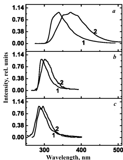
Fig. 3. Normalized fluorescence spectra of (a) tryptophan, (b) tyrosine, and (c) phenyl alanine: (1) powder specimens and (2) aqueous solutions
