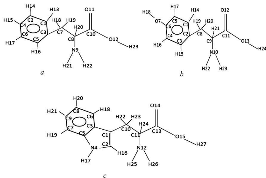
Fig. 1. Structures of (a) phenyl alanine, (b) tyrosine, and (c) tryptophan molecules
