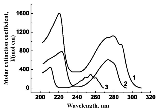
Fig. 2. Spectral dependences of the molar extinction coefficients for aqueous solutions of the aromatic amino acids: (1) tryptophan, (2) tyrosine, and (3) phenyl alanine
