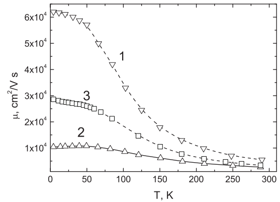
Fig. 3. Temperature dependences of the Hall mobility of electrons in the structures with different doping concentrations N_S , 10 11 cm -2 : 1 – 5.4; 2 – 17.5; 3 – 22
