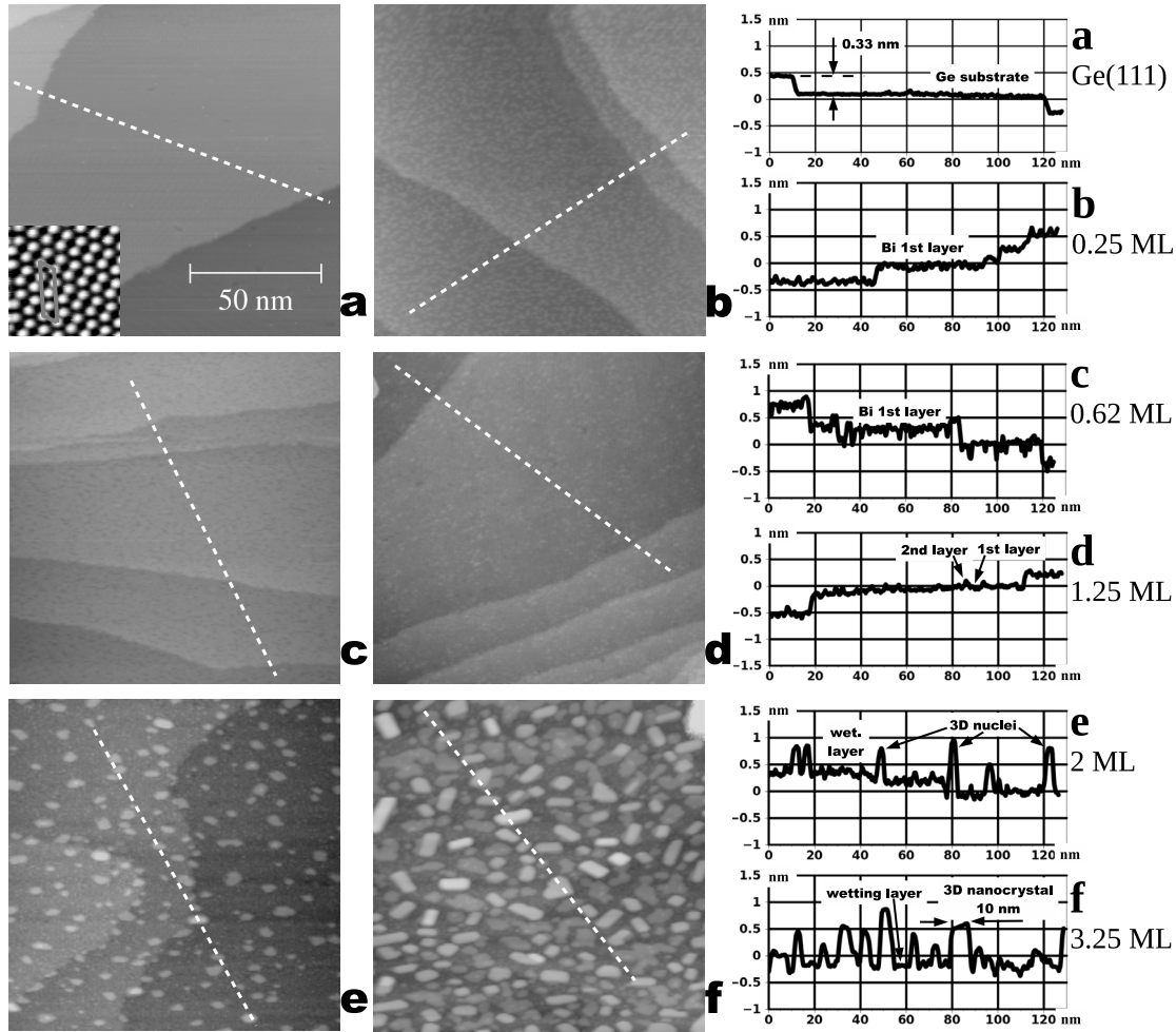
Fig. 1. Growth stage I: From the atomically flat Ge(111)-c( 2 \times 8 ) substrate to a nanocrystalline Bi film. All STM images are 125 \text{ nm} \times 125 \text{ nm} , specimen bias voltages are: a ) +1 V; b ) +2.5 V; c ) -2 V; d ) -2 V; e ) +1 V; f ) +2 V. The full grey-scale range corresponds to the 2.7 nm height difference between black and white. The right-most column contains cross-sections, which were obtained as height vs distance curves along white dashed lines within corresponding images. Every cross-section is labeled by the same letter as the image, in which it was taken, and by the deposited amount of Bi (in monolayers). Different cross-sections do not share any common height reference point, only the height differences can be compared. The inset in ( a ) is the atomic resolution image, showing a representative 6 \text{ nm} \times 6 \text{ nm} area on the top of the atomically flat terrace, with the c( 2 \times 8 ) unit cell outlined in grey. See the text for the discussion
