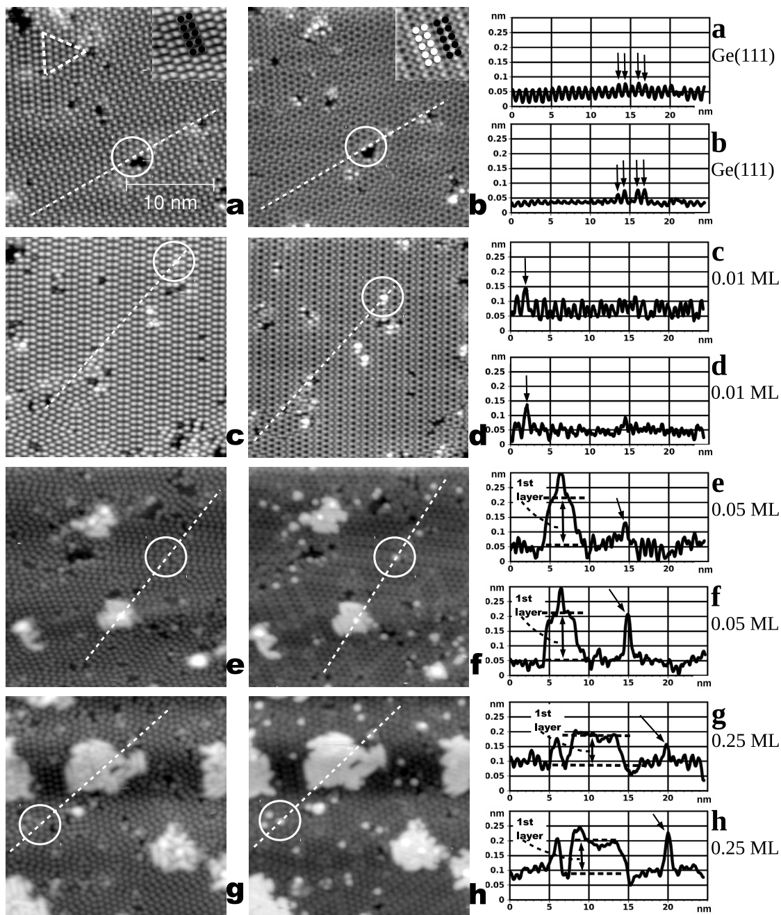
Fig. 5. Evolution of annealed submonolayer Bi films on Ge(111) as \theta_{\text{Bi}} is varied from 0 to 0.25 ML. All STM images are 25 \text{ nm} \times 25 \text{ nm} , the images within pairs a-b , c-d , e-f and g-h were obtained on the same surface areas of the corresponding specimens (small shifts are due to residual thermal drift). Panels a , c , e and g contain the images of empty states obtained with +2 V specimen bias voltage; panels b , d , f and h contain the images of occupied states obtained with -2 V specimen bias voltage. The right-most column contains cross-sections, which were obtained as height vs distance curves along white dashed lines within corresponding images. Every cross-section is labeled by the same letter as the image, in which it was taken, and by the deposited amount of Bi (in monolayers). The cross-sections are presented on similar vertical and horizontal scales to allow the comparison of height differences (no common height reference point). See the text for the discussion
