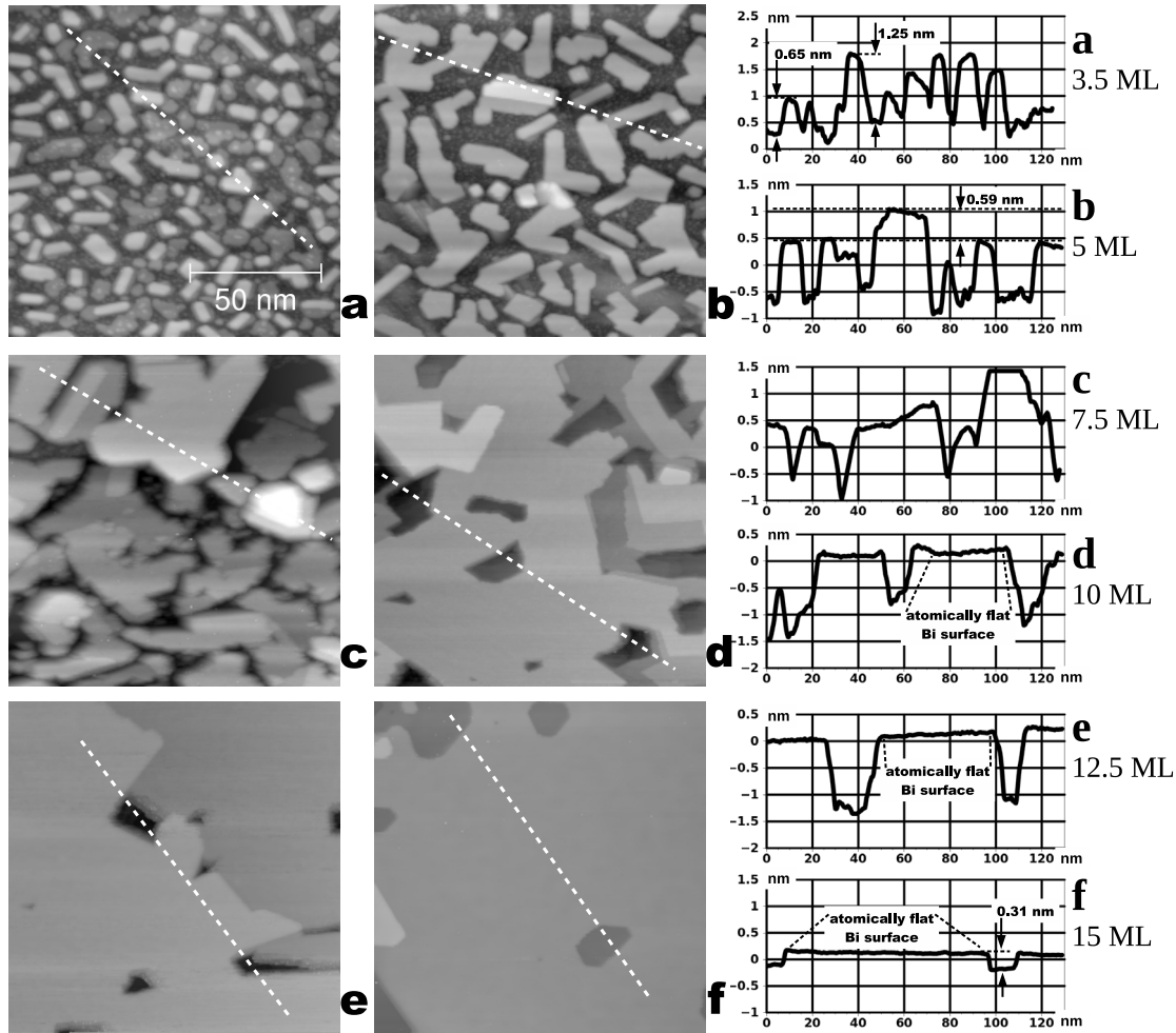
Fig. 2. Growth stage II: From the nanocrystalline to atomically flat Bi film. All STM images are 125 \text{ nm} \times 125 \text{ nm} , specimen bias voltages are: a) +2 V; b) -1 V; c) -0.5 V; d) +0.1 V; e) +0.1 V; f) -2 V. The full grey-scale range corresponds to the 2.7 nm height difference between black and white. The right-most column contains cross-sections, which were obtained as height vs distance curves along white dashed lines within corresponding images. Every cross-section is labeled by the same letter as the image, in which it was taken, and by the deposited amount of Bi (in monolayers). Different cross-sections do not share any common height reference point, only the height differences can be compared. See the text for the discussion
