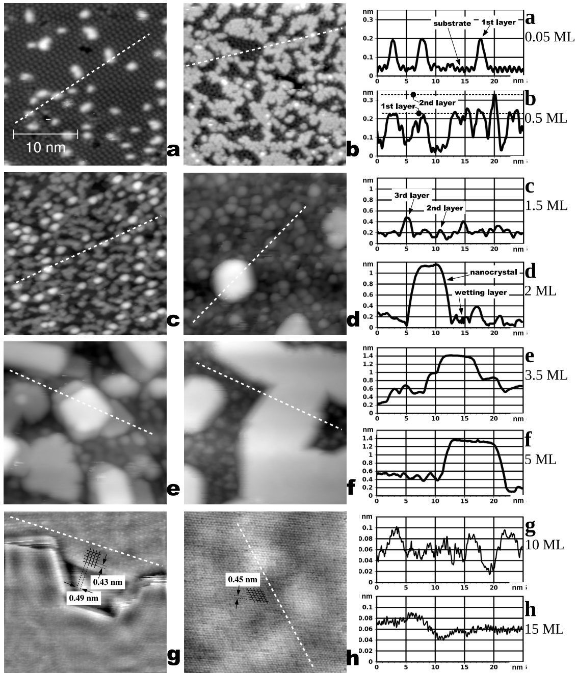
Fig. 3. Bi film growth on Ge(111)-c(2 × 8) on atomic scale. All STM images are 25 nm × 25 nm, specimen bias voltages are: a) +2.5 V; b) -2 V; c) -2 V; d) -2.5 V; e) +2 V; f) -1 V; g) +0.05 V; h) +0.01 V. The right-most column contains the cross-sections, which were obtained as height vs distance curves along white dashed lines within corresponding images. Every cross-section is labeled by the same letter as the image, in which it was taken, and by the deposited amount of Bi (in monolayers). a-d) formation of the wetting layer; d) nucleation of nanocrystals; e-f) growth and coarsening of nanocrystals; g-h) transition to a continuous film and the surface flattening
