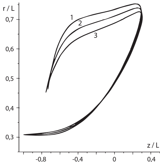
Fig. 3. Trajectory projections for particles with identical masses that start from the same position in the radial gap with various radial velocities v_r/v_0 = -0.02 (1), 0 (2), and 0.02 (3)
