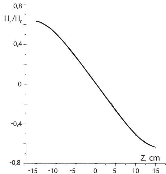
Fig. 2. Distribution of the H_z component of a magnetic field at r/L = 0.25
