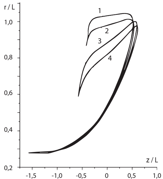
Fig. 1. Trajectory projections in the plane (r, z) for two particles with close masses ( M_1 < M_2 ), which start from the same radius. M_1 : v_r/v_0 = 3 \times 10^{-2} (1) and -3 \times 10^{-2} (2); M_2 : v_r/v_0 = 3 \times 10^{-2} (3) and -3 \times 10^{-2} (4)
