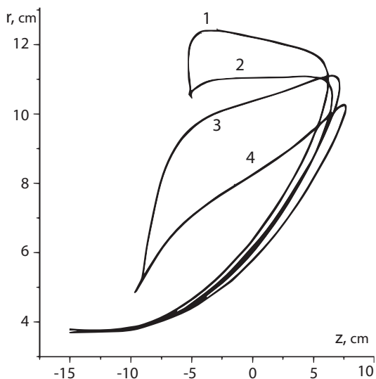
Fig. 4. Trajectory projections in the plane (r, z) for particles with different masses in the magnetic field of two coils. The field distribution is described by formulas (1) and (2). The parameter p_t = 0.19 (curves 1 and 2) and 0.21 (curves 3 and 4)
