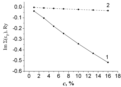
Fig. 6. Dependences of the (1) total imaginary part of the mass operator of Green's function for graphene and (2) its partial 2p_z component on the nitrogen impurity concentration c
