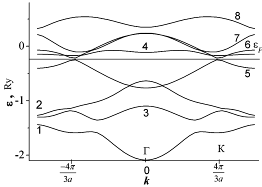
Fig. 1. Dependences of the electron energy in pure graphene on the absolute value of wave vector \mathbf{k} for the energy bands 2s (1 and 2), 2p_x (3 and 4), 2p_z (5 and 6), and 2p_y (7 and 8)
