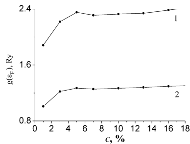
Fig. 7. Dependences of the (1) total electron density of states in graphene at the Fermi level and (2) its partial 2p_z component on the nitrogen impurity concentration c
