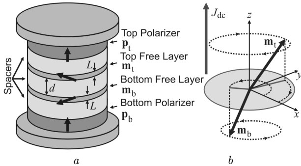
Fig. 3. (a) Layout of the symmetric dual-free-layer STNO consisting of four magnetic layers: two inner FLs of thickness L and two outer PLs separated by the GMR spacer of thickness d . (b) The torques acting on the magnetization vectors of the FLs in the STNO driven by the transverse bias dc current of the density J_{dc}
