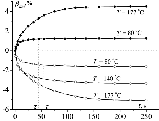
Fig. 1. Time dependences of the relative relaxation amplitudes \beta_{12} (solid circles) and \beta_{13} (hollow circles)
