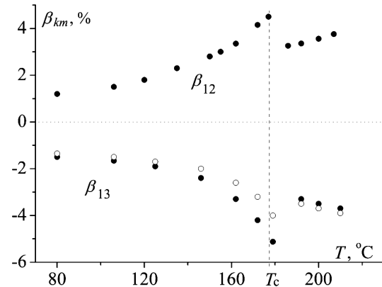
Fig. 2. Temperature anomalies of the relative relaxation amplitudes \beta_{km} : experimental (solid circles) and calculated values (hollow circles)
