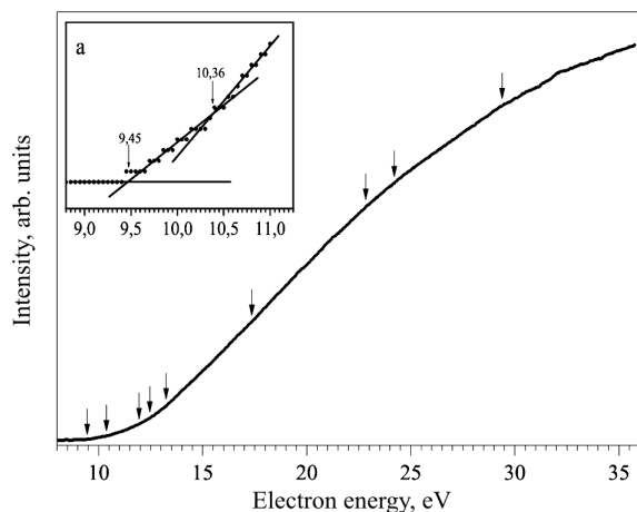
Fig. 5. Energy dependence of the total cross-section for the formation of positive ions in sulfur vapor. An example of the approximation of linear sections is shown in the inset
