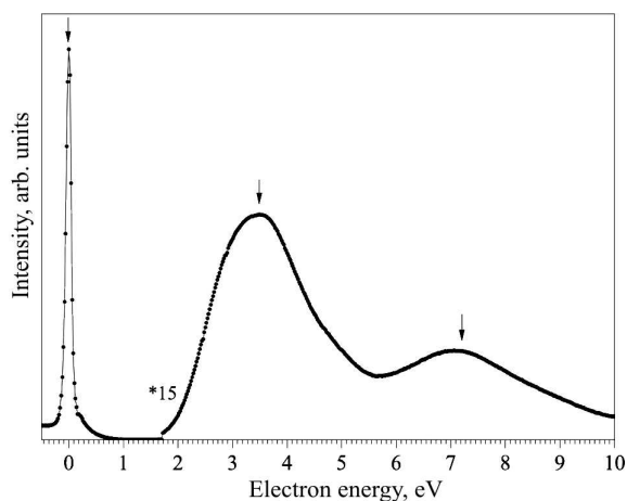
Fig. 6. Energy dependence of the total cross-section for the formation of negative sulfur ions
