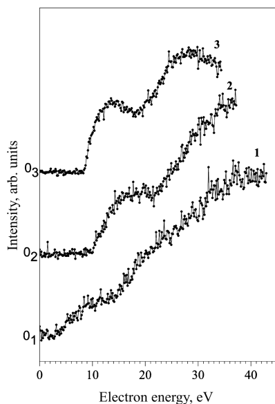
Fig. 2. OEFs of atomic spectral lines: sulfur (1, \lambda = 469.4/.5/.6 nm), selenium (2, \lambda = 207.5 nm), and tellurium (3, \lambda = 225.9 nm)
