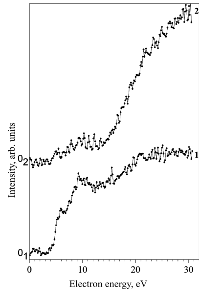
Fig. 3. OEFs of spectral lines of single-charged sulfur ions at \lambda = 393.3 (1) and 542.8/543.2/545.3 nm (2)
