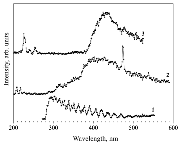
Fig. 1. Emission spectra of S (1, E_3 = 8 eV), Se (2, E_3 = 30 eV), and Te (3, E_3 = 10 eV) vapors
