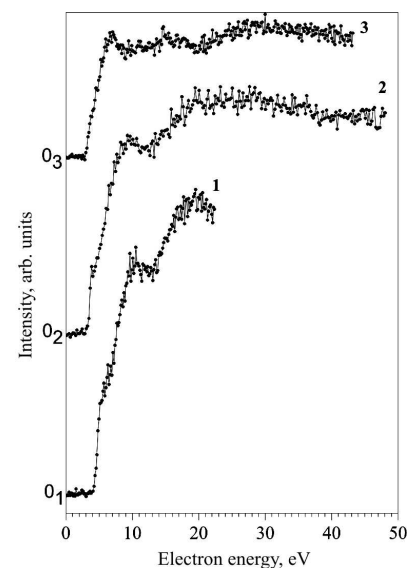
Fig. 4. OEFs of spectral molecular emissions: sulfur (1, \lambda = 376 nm), selenium (2, \lambda = 383 nm), and tellurium (3, \lambda = 430 nm)
