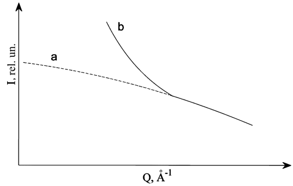
Classical (a) and anomalous (b) asymptotics of the neutron scattering intensity
