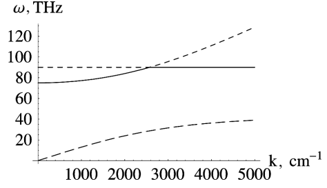
Fig. 1. Low-frequency transverse modes for NaF
