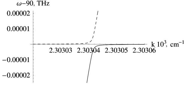
Fig. 2. Mutual approach of upper phonon-polaritons in NaF
