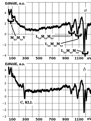
Fig. 6. Auger electron spectra of the Ge(111) substrate under clean (a) and carbon-contaminated (b) conditions. The EdN/dE spectra were obtained in the analog differentiation mode. The peaks in the spectra are designated according to their respective Auger transitions, which were excited by 3-keV primary electrons
