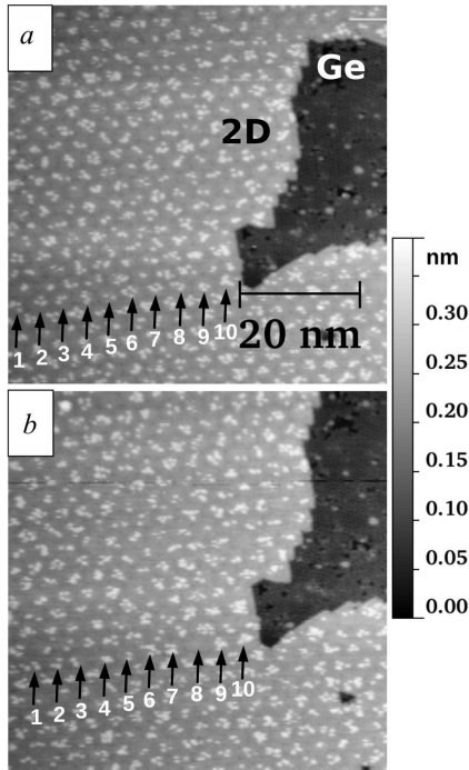
Fig. 4. Two consecutive STM images obtained on the same surface area ( 62 \times 62 nm) of the Ge(111) sample showing an extended patch covered by the 2D overlayer. There is some small noticeable shift between the images due to the thermal drift and the STM piezoscanner creep). Sample bias voltage: -2.5 V, tunneling current: 0.3 nA. 10 identical superlattice sites are marked by numbered arrows on both images
