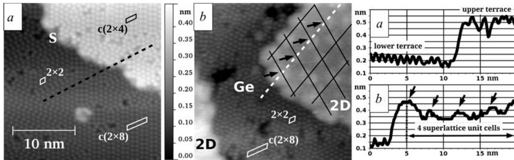
Fig. 2. STM images in atomic resolution ( 25 \times 25 nm field of view) of: pure reconstructed Ge(111) surface, sample bias voltage: +2.5 V; tunneling current: 0.3 nA. c(2 \times 8) , c(2 \times 4) and 2 \times 2 superstructures are present, their unit cells are outlined and marked, correspondingly; a single atomic step between the upper and lower neighboring terraces is designated by “S” a . The mixture of pure Ge and a 2D hexagonal overlayer, sample bias voltage: +2 V; tunneling current: 0.3 nA, outlined are the 2 \times 2 and c(2 \times 8) unit cells on the pure Ge area and the 2D superlattice formed by height maxima (black mesh). On the right are height-distance cross-sections along dashed lines in corresponding panels. The height maxima lying along the cross-section line are designated by small black arrows b . The grey scale to a height conversion ruler is common for both images
