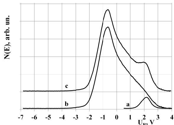
Fig. 1. PESs for a typical photocathode excited in various regimes: h\nu = 3.1 eV (a), h\nu = 10.2 eV (b), and h\nu = 10.2 and 3.1 eV (c) simultaneously
