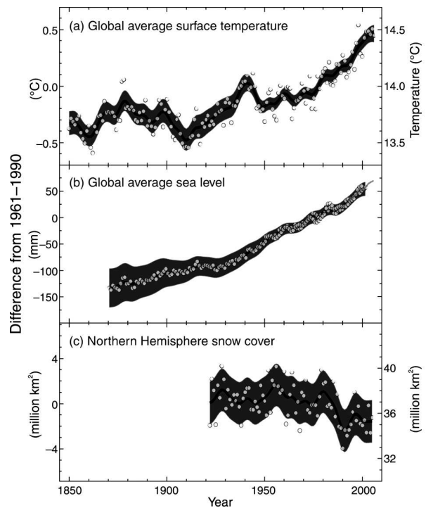
Fig. 1. Observed changes in the global average surface temperature (a); global average sea level from tide gauge (blue) and satellite (red) data (b) and the Northern Hemisphere snow cover for March-April (Taken from work [6]) (c)
