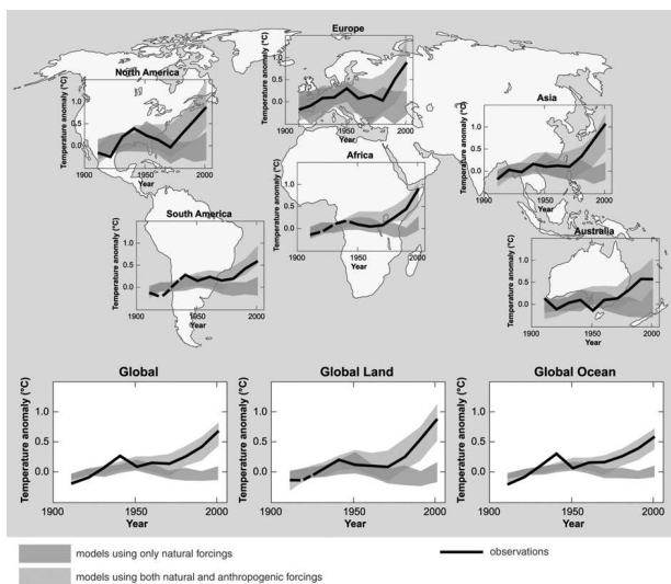
Fig. 3. Comparison of the observed continental- and global-scale changes in the surface temperature with the results simulated by climate models using either natural or both natural and anthropogenic forcings. (Taken from work [6])
