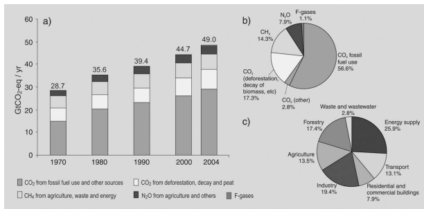
Fig. 2. Global annual emissions of anthropogenic greenhouse gases (GHGs) from 1970 to 2004 (a). Share of different anthropogenic GHGs in total emissions in 2004 in terms of carbon dioxide equivalents (CO 2 -eq) (b). Share of different sectors in total anthropogenic GHG emissions in 2004 in terms of CO 2 -eq. (Forestry includes deforestation) (Taken from work [6]) (c)
