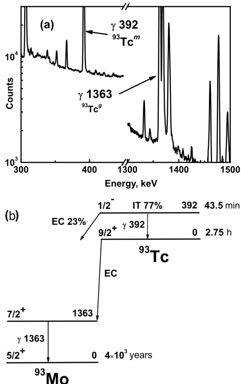
Fig. 1. Fragments of the spectrum (a) and decay schemes for the ^{93}\text{Tc}^{m,g} nucleus (b)
