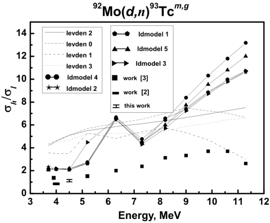
Fig. 5. The same as in Fig. 4, but for the nuclear reaction ^{92}\text{Mo}(d,n)^{93}\text{Tc}^{m,g}
