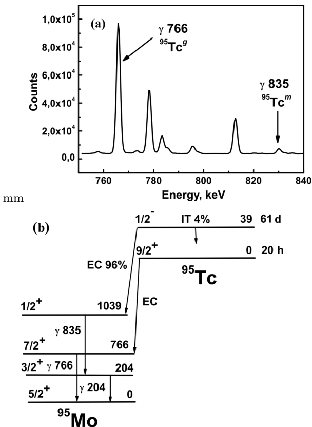
Fig. 2. The same as in Fig. 1, but for the ^{95}\text{Tc}^{m,g} nucleus
