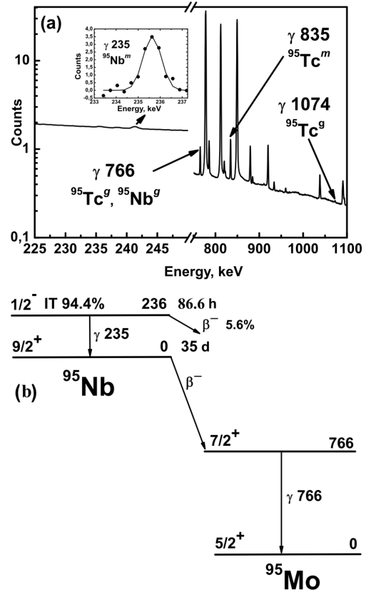
Fig. 3. The same as in Fig. 1, but for the ^{95}\text{Nb}^{m,g} nucleus
