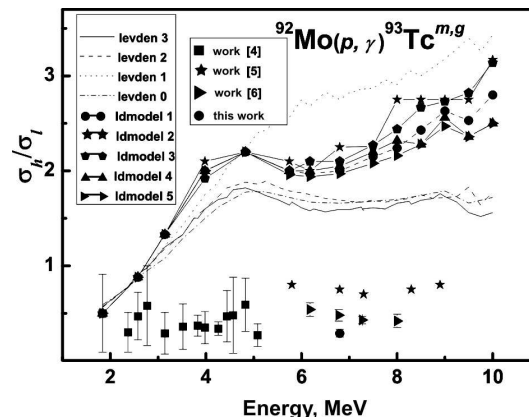
Fig. 4. Experimental and theoretical ICSRs for the nuclear reaction ^{92}\text{Mo}(p, \gamma)^{93}\text{Tc}^{m,g} . To describe the level density, the following models were used: ldmodel = 1 and levden = 2 correspond to the model of constant temperature (CT) and Fermi gas (FG) (CT + FG) [29]; levden = 3 to the microscopic combinatorial model (HFBM) [30]; levden = 1 to the generalized superfluid model (GSM) [31, 32]; levden = 0 to the improved superfluid model (EGSM) [33]; ldmodel = 2 to the back-shifted Fermi gas model (BFM) [34]; ldmodel = 3 to the generalized superfluid model (GSM) [35, 36]; ldmodel = 4 to the microscopic model [37]; and ldmodel = 5 to the microscopic model [38]
