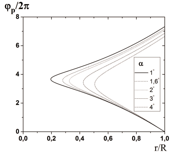
Fig. 6. Dependence of the phase change along the inclined ray trajectory at the parabolic density profile (6) with \gamma = 2 for various \alpha
