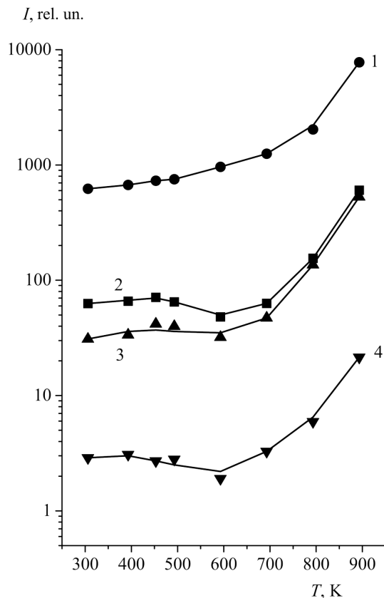
Fig. 8. Temperature dependences of the emission intensity of positive oxygen-containing secondary ions sputtered from the LaNi 5 surface. Measurements were carried out under the residual partial hydrogen pressure and at the current density of primary ions j = 4.5 \mu\text{A}/\text{cm}^2 : (1) \text{LaO}^+ , (2) \text{La}_2\text{O}^+ , (3) \text{La}_2\text{O}_2^+ , and (4) \text{La}^{58}\text{NiO}^+
