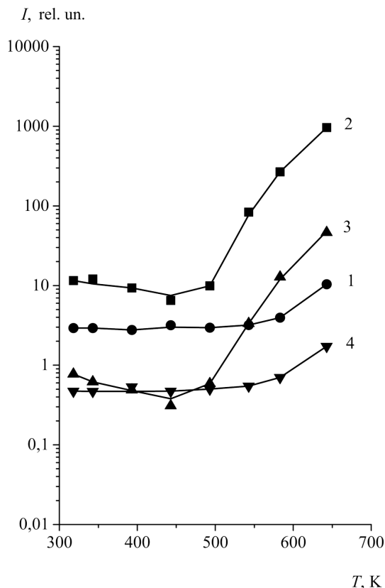
Fig. 7. Temperature dependences of the emission intensity of negative carbon-containing secondary ions sputtered from the LaNi 5 surface. Measurements were carried out under the residual partial hydrogen pressure and at the current density of primary ions j = 4.5 \mu\text{A}/\text{cm}^2 : (1) ^{58}\text{NiC}^- , (2) ^{58}\text{NiC}_2^- , (3) \text{LaC}_2^- , and (4) \text{LaC}_4^-
