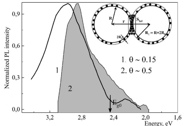
Fig. 3. PL spectra of a film of N particles with the cover fraction \theta = 0.15 (1) and film F1 (2). The arrow marks the energy position of the forbidden gap in CdS, E_{g0} \approx 2.44 eV. The inset illustrates a contact between two N particles
