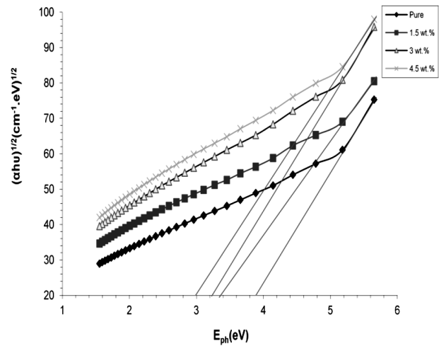
Fig. 3. Variation of the energy band gap for allowed indirect transitions of (CMC-starch-CuO) nanocomposites
