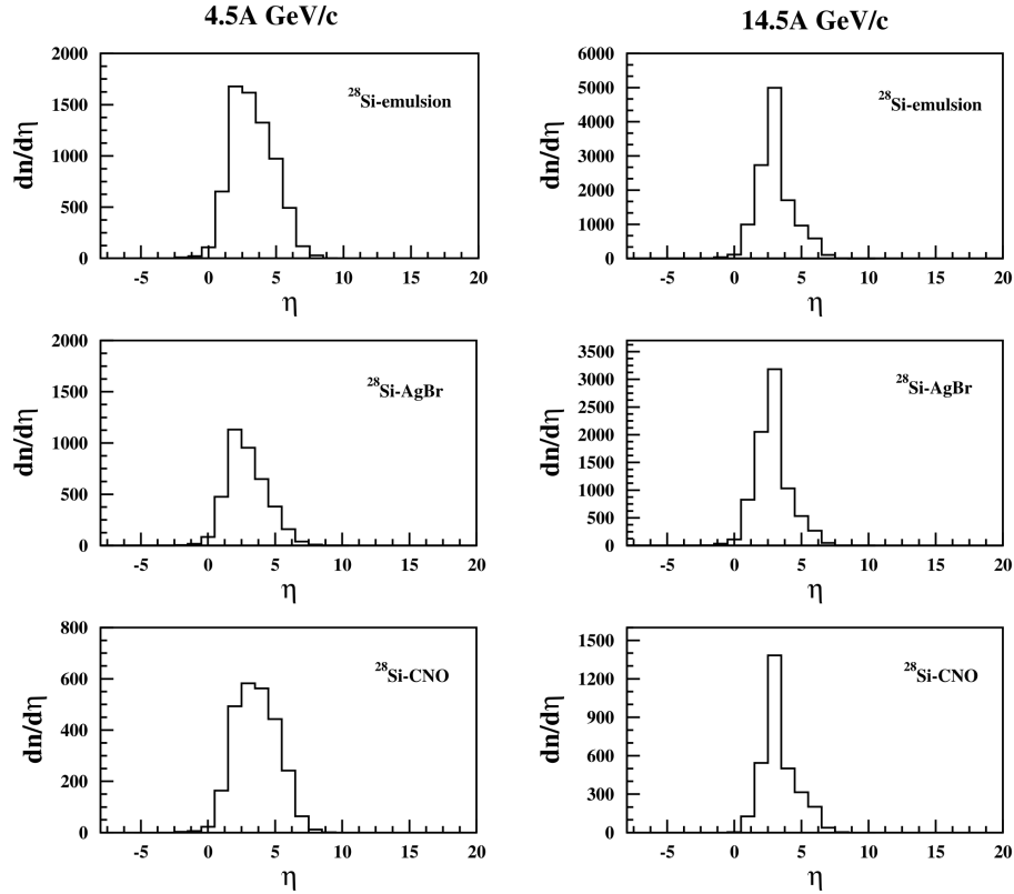
Fig. 1. Rapidity distributions of the interactions of ^{28}\text{Si} with various targets at 4.5A and 14.5A GeV/c
