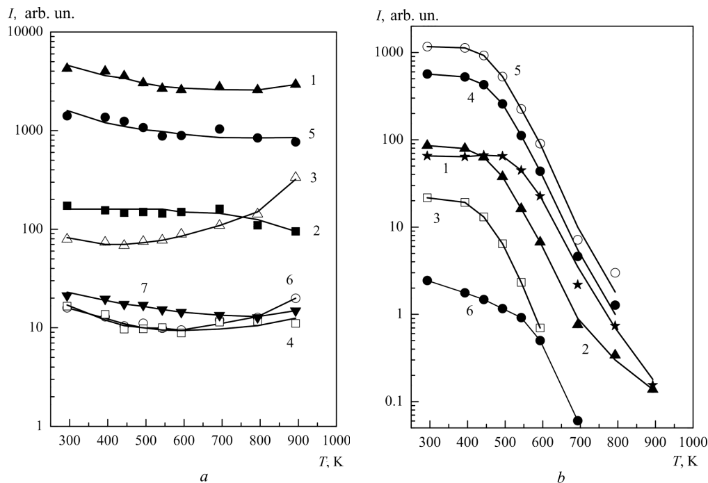
Fig. 4. Temperature dependences of the emission intensity for positive secondary ions sputtered from the surface of the TiFe alloy specimen at the hydrogen partial pressure P_{\text{H}_2} = 3.5 \times 10^{-4} Pa and a primary beam current density of 6.0 \mu\text{A}/\text{cm}^2 ; panel a: ^{48}\text{Ti}^+ (1), ^{56}\text{Fe}^+ (2), ^{48}\text{TiO}^+ (3), ^{56}\text{FeO}^+ (4), \text{TiFe}^+ ( m = 104 amu) (5), \text{TiFeO}^+ ( m = 120 amu) (6), and ^{48}\text{TiC}^+ (7); panel b: \text{H}^+ (1), ^{48}\text{TiH}^+ (2), ^{56}\text{FeH}^+ (3), \text{TiFeH}^+ ( m = 105 amu) (4), ^{48}\text{Ti}_2\text{H}^+ (5), and \text{CH}^+ (6)
