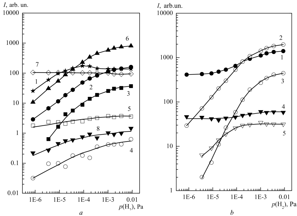
Fig. 3. Dependences of the emission intensity on the hydrogen partial pressure in a target chamber for positive secondary ions sputtered from the TiFe alloy surface at the temperature T = 293 K and a primary beam current density of 6.0 \mu\text{A}/\text{cm}^2 ; panel a : \text{H}^+ (1), ^{50}\text{TiH}^+ (2), ^{56}\text{FeH}^+ (3), ^{50}\text{TiOH}^+ (4), ^{56}\text{FeOH}^+ (5), \text{TiFeH}^+ ( m = 105 amu) (6), ^{48}\text{TiO}^+ (7), and \text{CH}^+ (8); panel b : ^{48}\text{Ti}_2^+ (1), ^{48}\text{Ti}_2\text{H}^+ (2), ^{48}\text{Ti}_2\text{H}_2^+ (3), ^{48}\text{Ti}_2\text{C}^+ (4), and ^{48}\text{Ti}_2\text{CH}^+ (5)
