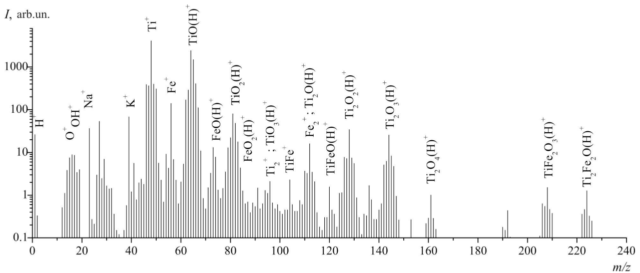
Fig. 1. Panoramic mass spectrum of positive secondary ions sputtered from the surface of a specimen of TiFe alloy at room temperature in the residual vacuum and at a primary beam current density of 1.5 \mu\text{A}/\text{cm}^2
