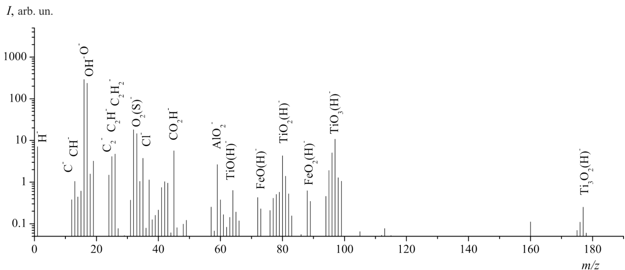
Fig. 2. Panoramic mass spectrum of negative secondary ions sputtered from the surface of a specimen of TiFe alloy at room temperature in the residual vacuum, and at a primary beam current density of 1.5 \mu\text{A}/\text{cm}^2
