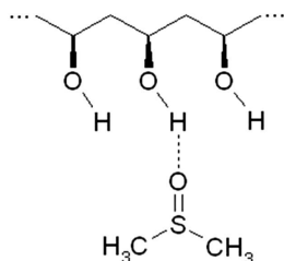
Fig. 2. Diagram of hydrogen bond formation between a monomer of a PVA macromolecule and a DMSO molecule
