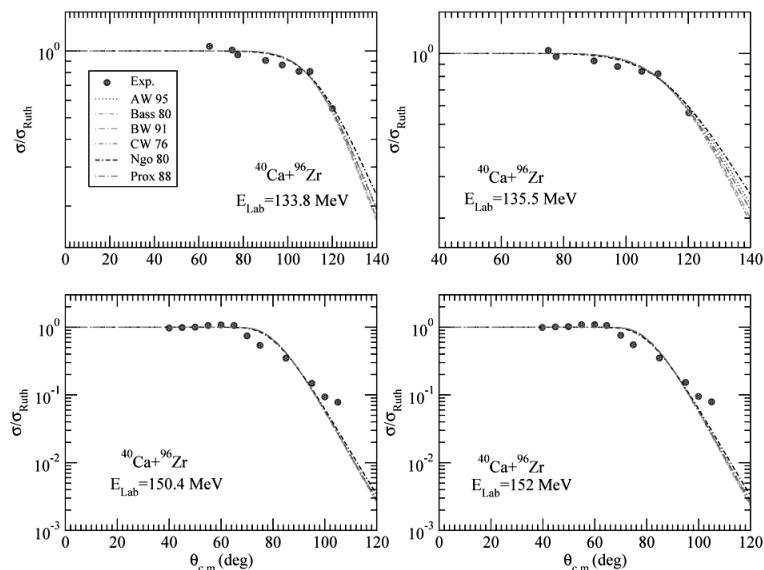
Fig. 5. The same as Fig. 2, but for the ^{40}\text{Ca} + ^{96}\text{Zr} reaction at E_{lab} = 133.8 , 135.5, 150.4, and 152 MeV. The experimental data have been taken from [4, 5]
