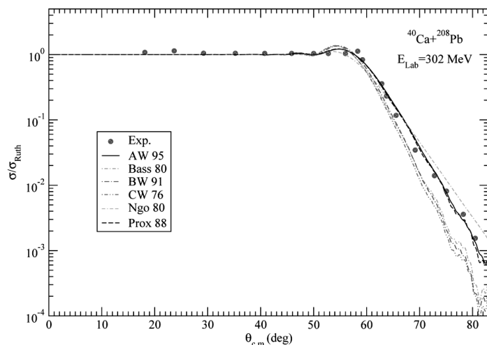
Fig. 6. The same as Fig. 2, but for the ^{40}\text{Ca} + ^{208}\text{Pb} reaction at E_{lab} = 302 MeV. The experimental data have been taken from [6]
