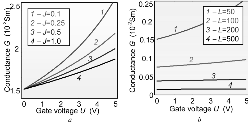
Fig. 14. Dependences of the conductance G on the gate voltage U calculated (a) for various binding energies J (indicated in the legend in \text{J/m}^2 units) at L = 50 \text{ nm} and (b) for various channel lengths L (indicated in the legend in \text{nm} units) at J = 0.5 \text{ J/m}^2 . Adapted from [A.N. Morozovska, A.I. Kurchak, M.V. Strikha. Phys. Rev. Appl. 8 , 054004 (2017)] with permission from AIP Publishing for the authors' artwork
