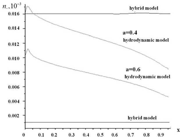
Fig. 8. Comparison between the results of numerical calculations for the electron concentration in the discharge gap in the hydrodynamic and hybrid models
