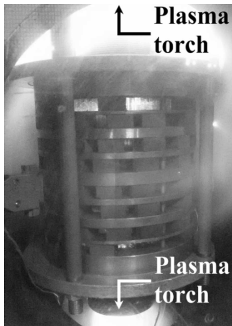
Fig. 5. Image of the accelerator operating in the high-discharge mode. Plasma torches are visible at system's ends
