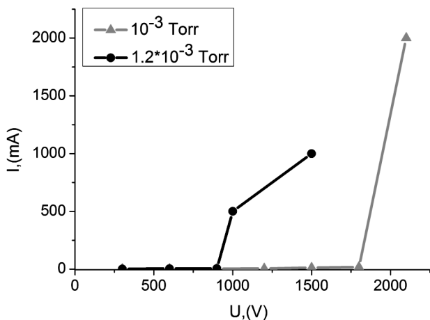
Fig. 3. CVCs of the accelerator for various working gas pressures in the high-current mode
