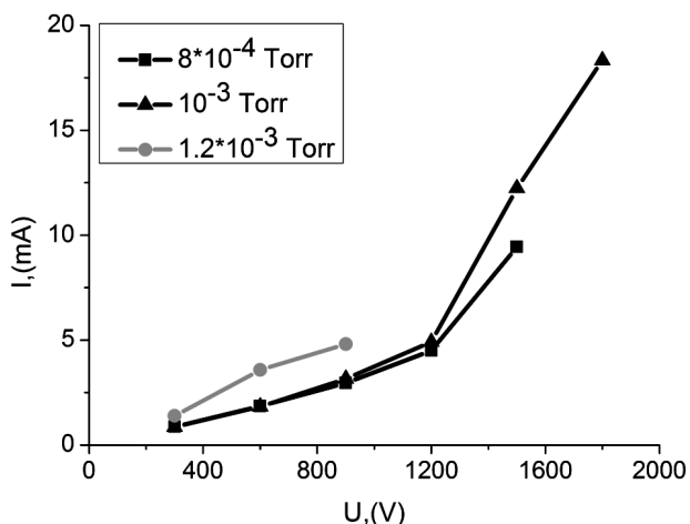
Fig. 4. CVCs of the accelerator for various working gas pressures in the low-current mode
