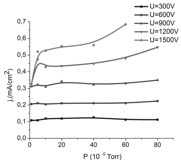
Fig. 2. Dependences of the discharge current density on the working gas pressure for various voltages across a discharge gap in the low-current mode
