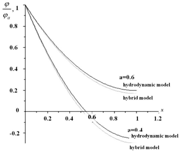
Fig. 7. Comparison between the results of numerical calculations for the potential distribution in the discharge gap in the hydrodynamic and hybrid models
