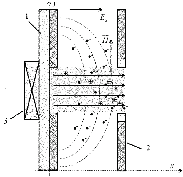
Fig. 6. Plasma accelerator model: anode (1), cathode (2), magnetic system (3). Dashed curves denote power lines of the magnetic field. Arrows indicate the ion acceleration direction
