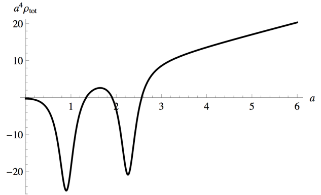
Fig. 4. Total energy density \rho_{\text{tot}} multiplied by a^4 for the quantum source Q (24) versus the scale factor a for n = 2
