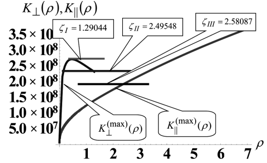
Fig. 7. Projections of the maximum values of the orthogonal, K_{\perp}^{(\max)}(\rho) , and parallel, K_{\parallel}^{(\max)}(\rho) , components of the coefficient K(\omega, \rho) of light absorption by a spheroidal metal nanoparticle on the plane (K, \rho) , and the half-widths of the functions P_i(\rho) , i = I, II, III
