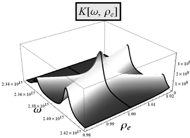
Fig. 2. Dependence K(\omega, \rho_e) of the coefficient of light absorption by a spheroidal metal nanoparticle on its form (the parameter \rho_e ) and the light frequency \omega
