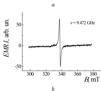
Fig. 3. RTEM spectrum of a specimen functionalized with a mixture of sulfuric and nitric acids: full spectrum ( a ) and the region in the vicinity of g = 2.00 ( b )
