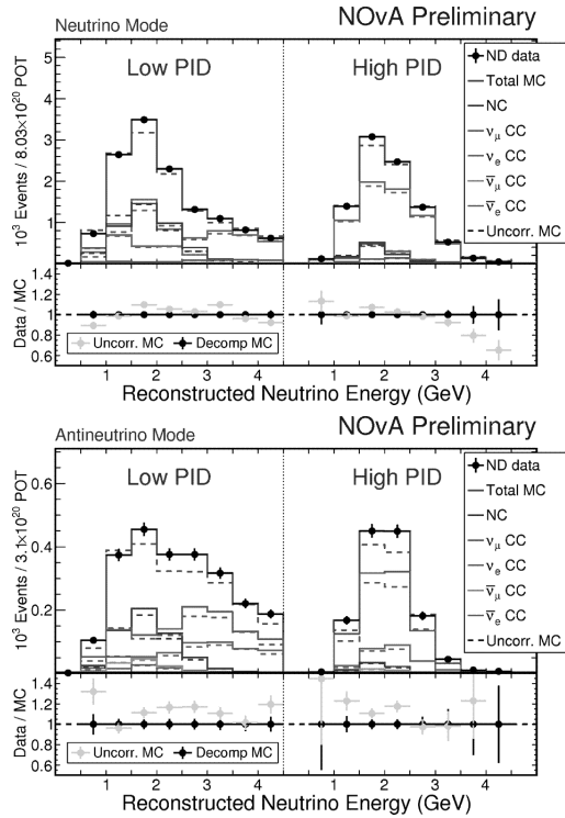
Fig. 4. ND selected \nu_e (top) and \bar{\nu}_e (bottom) reconstructed energy data (black dots), uncorrected simulation (dashed red) and data-driven correction (solid red). The selection is decomposed (broken down) into NC (blue), \nu_\mu/\bar{\nu}_\mu CC (dark/light green) and \nu_e/\bar{\nu}_e CC (light/dark magenta). Binned in two PID bins, which are correlated to lower and higher purities of \nu_e + \bar{\nu}_e
