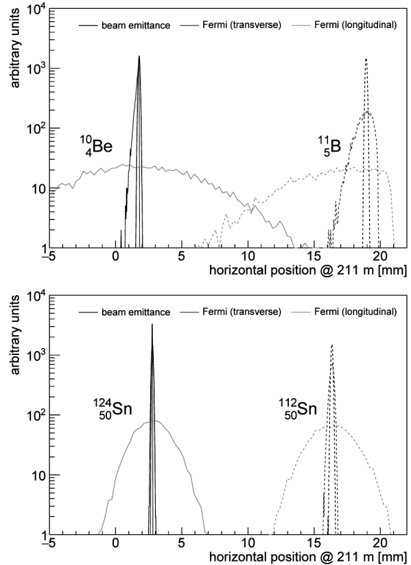
Fig. 6. Effects of the beam emittance and the Fermi motion on the fragment position in the AFP for selected light (top) and heavy (bottom) nuclei
