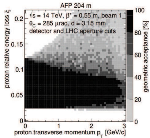
Fig. 3. Geometric acceptance of the AFP detectors for forward protons
