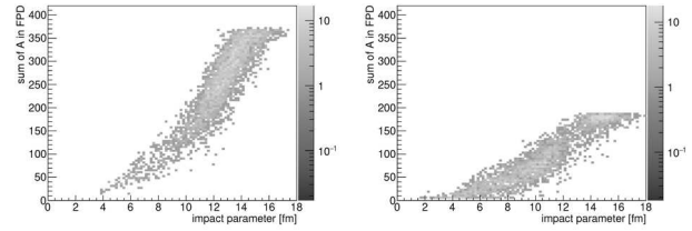
Fig. 11. Correlation between the collision impact parameter and the sum of mass numbers of fragments produced within the acceptance of forward proton detectors for double-tag (left) and single-tag (right) (see text)
