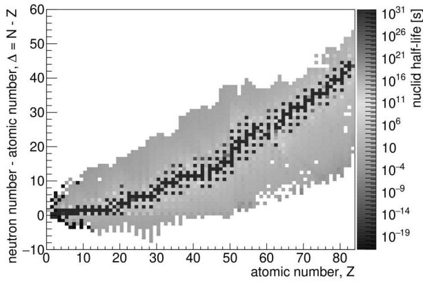
Fig. 4. Half-life time of the known nuclei
