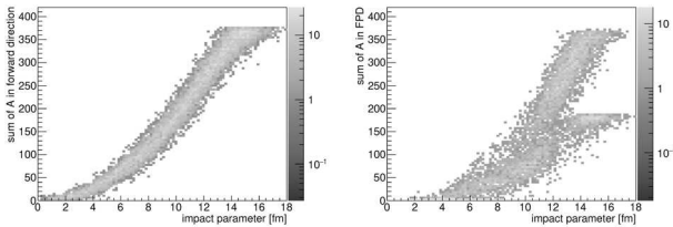
Fig. 9. Correlation between the collision impact parameter and the sum of mass numbers of: all produced fragments (left), fragments produced within the acceptance of forward proton detectors (right)
