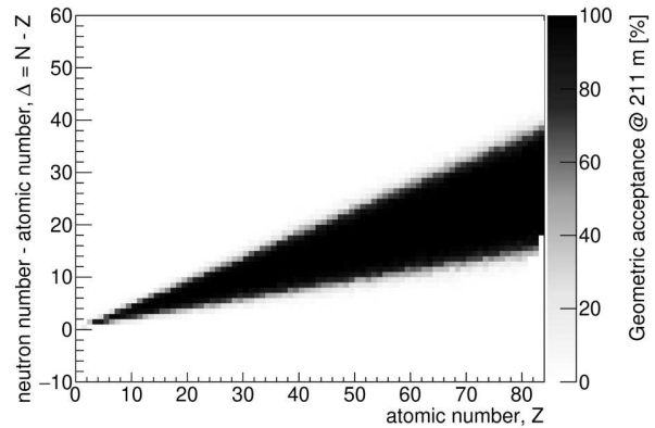
Fig. 7. AFP acceptance for nuclear fragments
