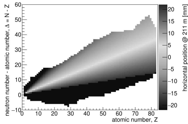
Fig. 5. Horizontal position of the nuclei at the distance of 211 m from the ATLAS interaction point
