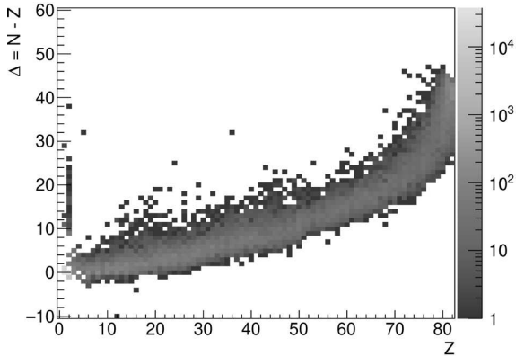
Fig. 8. Multiplicity of the nuclear fragments produced in Pb–Pb collisions simulated using DPMJET
