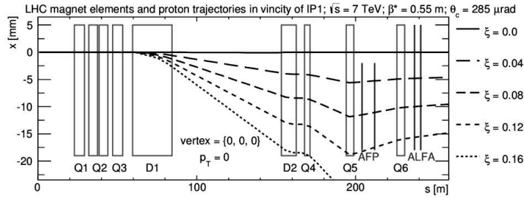
Fig. 2. Trajectories of forward protons in the LHC magnetic lattice. s is the distance from the interaction point along the nominal optics, x is the horizontal coordinate of a trajectory with respect to the nominal orbit, \xi is the relative energy loss of a forward proton
