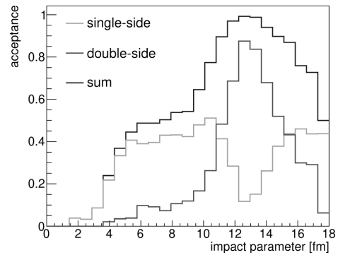
Fig. 12. Acceptance for events with nuclear fragments measured in forward proton detectors
