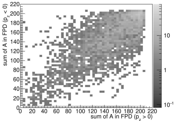
Fig. 10. Correlation between the sum of masses of fragments produced within the acceptance of forward proton detectors on the sides with positive and negative longitudinal momenta
