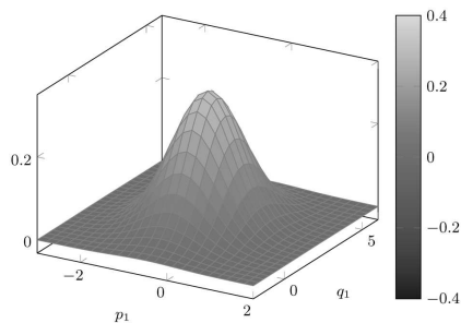
Fig. 1. Wigner Function (cut in q_1, p_1 ), Ground State
