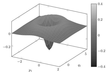
Fig. 2. Wigner Function (cut in q_1, p_1 ), First Excited State
