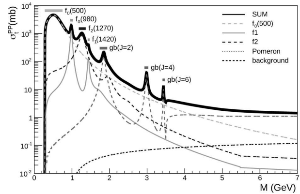
Fig. 2. Pomeron-pomeron total cross-section in CED calculated in Ref. [1]
