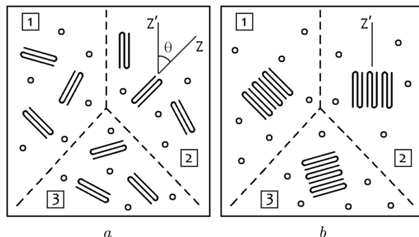
Fig. 5. Schematic diagrams of the structure of metulose aqueous solution at temperatures of 30^\circ\text{C} (a) and 75^\circ\text{C} (b)
