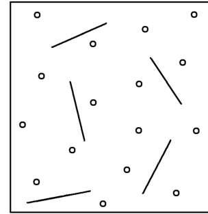
Fig. 1. Structural model for a solution of rod-like molecules
