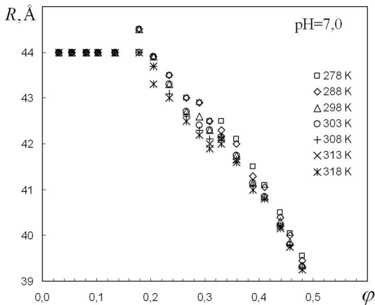
Fig. 4. Concentration dependences of the effective radius of albumin-I macromolecules along the isotherms at pH = 7.0 [21]
