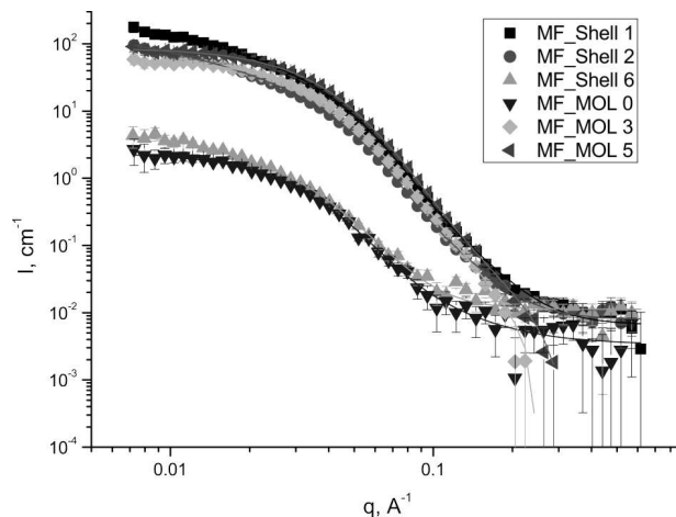
Fig. 5. SANS data (points) and the fit (curves) for the ferrofluids based on insulating transformer oils SHELL and MOL with electrodes without the dc electric field (0 kV/cm)
