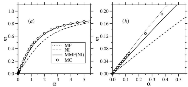
Fig. 3. The magnetization curve with \sigma = 0 and J = 0.5 : expanded scale ( a ); linear-response regime ( b ). The points are from MC simulations, and the lines are from theory: MF theory (dotted line); non-interacting (NI) spins (dashed line); MMF(NI) theory based on non-interacting spins (solid line)
