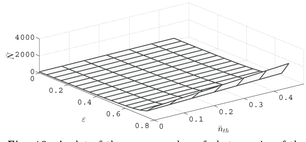
Fig. 13. A plot of the mean number of photon pairs of the cavity radiation (Eq. (65)) at the steady state for x = 0.03 , \kappa = 0.75 , \zeta = 0.03 , and A = 100
