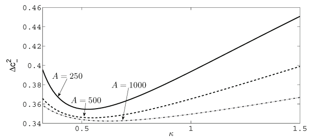
Fig. 8. Plots of the minus quadrature variance [Eq. (50)] of the two-mode cavity radiation at the steady state for x = 0.03 , \zeta = 0.01 , \varepsilon = 0.5 , \bar{n}_{\text{th}} = 0.15 , and for different values of A
