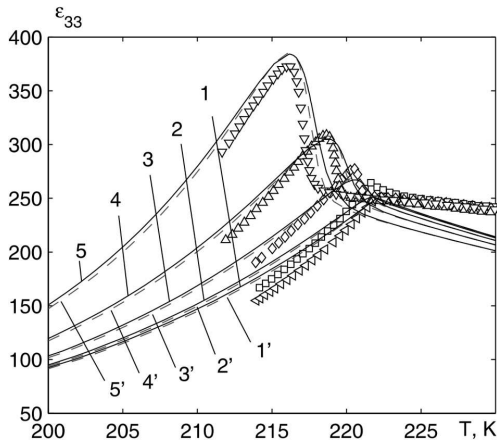
Fig. 9. Temperature dependences of the dielectric permittivity \epsilon_{33}^f at different values of the field strength E_3 (MV/m): 0.0 – 1 ( \nabla ); 1.0 – 2 ( \square ); 2.0 – 3 ( \diamond ); 3.0 – 4 ( \triangle ); 4.0 – 5 ( \nabla ) [7] and at the applied simultaneously longitudinal field E_2 = 0.07E_3 . Red dashed curves 1'–5' [25] of the permittivity \epsilon_{33}^c at the same values of E_3 and at the field E_2 \sim 0.05E_3 applied simultaneously
