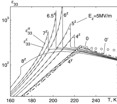
Fig. 8. Temperature dependences of the transverse dielectric permittivities of mechanically free \epsilon_{33}^f (solid lines) and clamped \epsilon_{33}^c (dashed lines) GPI crystals at different values of the fields E_2 and E_3 ; symbols \circ are experimental data [1] at the zero field
