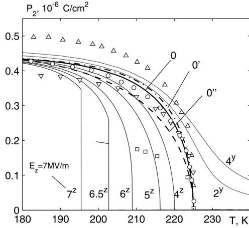
Fig. 2. Temperature dependences of the longitudinal polarization P_2 of GPI crystal at different values of the electric fields E_2 and E_3 . Curves 0 (the present result), 0' [17], 0'' [18], as well as symbols \circ [19], \Delta [1], \square [22], \nabla [16] correspond to zero field
