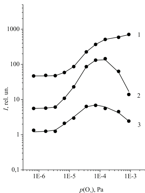
Fig. 7. Dependences of the emission intensity of various secondary polyatomic ions with nickel sputtered from the LaNi 5 surface at room temperature on the partial pressure of oxygen: 58 Ni 2 + (1), Ni 3 + (2, m/z = 176), and Ni 4 + (3, m/z = 234)
