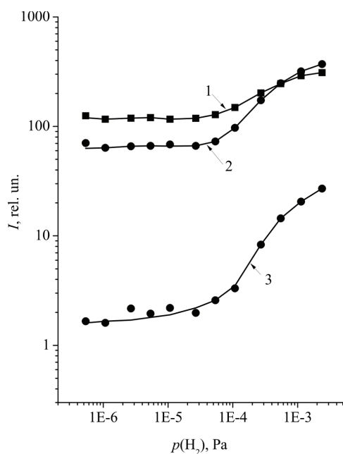
Fig. 8. Dependences of the emission intensity of various secondary polyatomic ions with nickel sputtered from the LaNi 5 surface at room temperature on the partial pressure of hydrogen: 58 Ni 2 - (1), Ni 3 - (2, m/z = 174), and Ni 4 - (3, m/z = 234)
